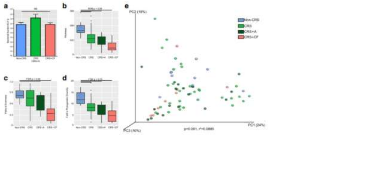
Figure 1: CRS patients and their microbiota
